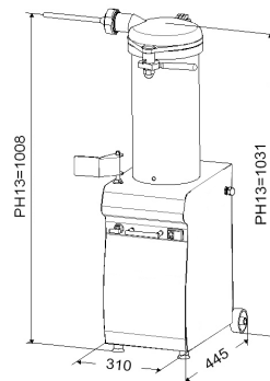
Dimension PH13
